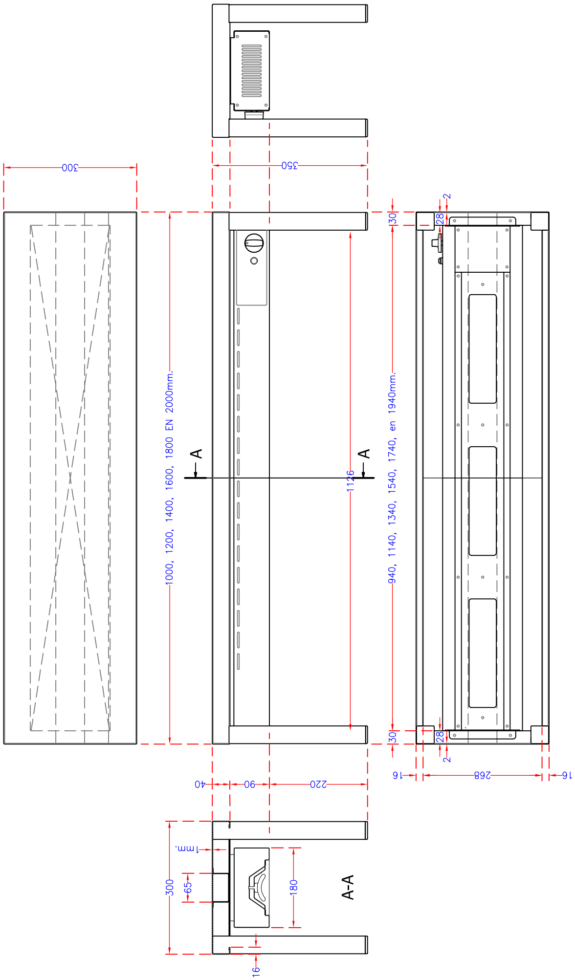
ETAGERES SINGLE + Heat strip brushed stainless steel 1mm.
